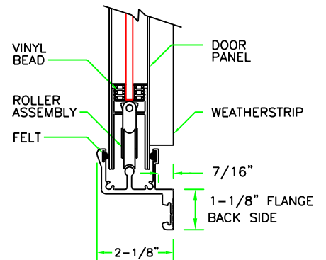
VIEW A (TYPICAL FOR SILL AND HEAD)
